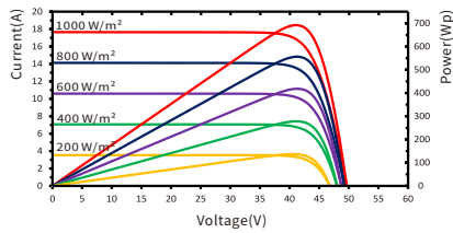
RSM132-8-690BHDG I-V characteristics at different irradiances
