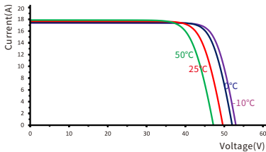
I-V characteristics at different temperatures (AM1.5, 1000W/m 2 )
